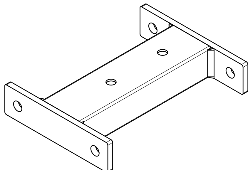
Foot Plate Crossmember
