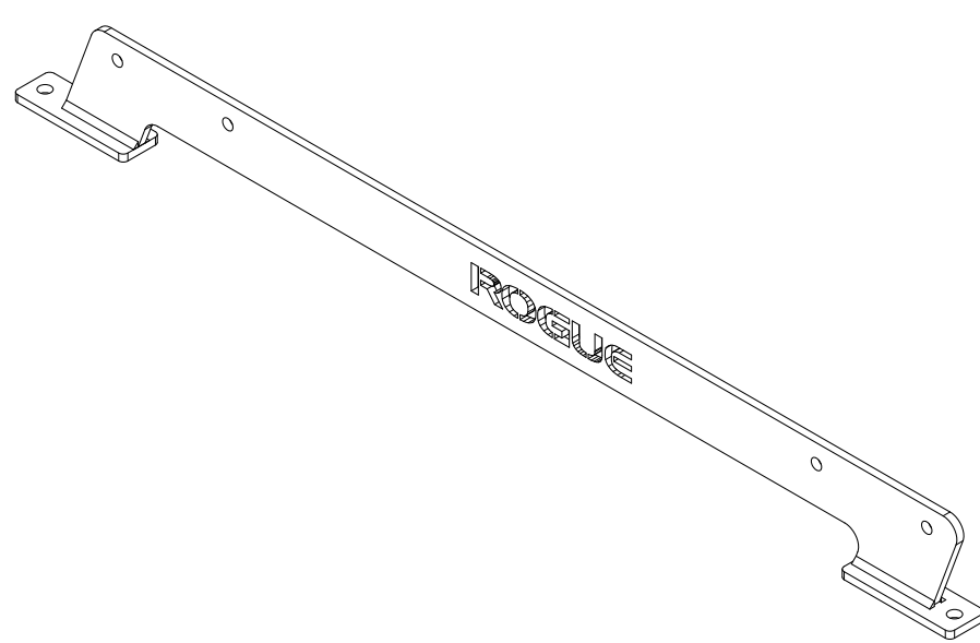
Floor Glute Side - LH
